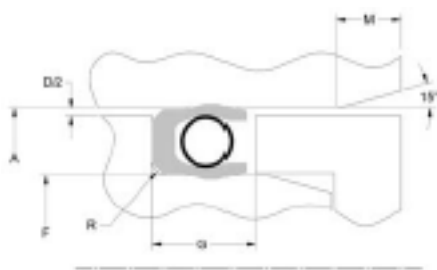
Seal Groove — Piston
