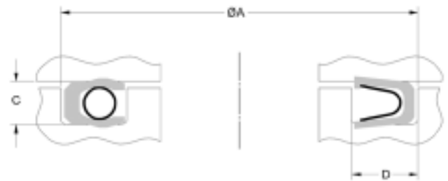
SFS (Static Face Seal) Finger Spring in Gland
