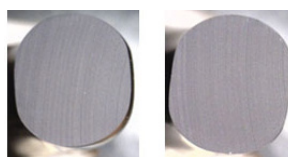
Test 1: Representative Seal Sections of Fusion™ 944 after ISO Test at 210°F (100°C) and 290 PSI (20 bar)/min Decompression Rate
