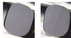
Test 4: Representative Seal Sections of Fusion™ 944 after ISO Test at 450°F (230°C) and 1,450 PSI (100 bar)/min Decompression Rate
