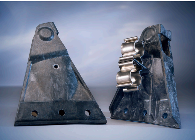
Compression Molded DLF Carbon/PEEK EBU Brackets
