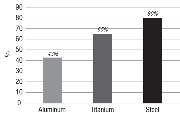
Xycomp® DLF™ density reduction vs. metal
