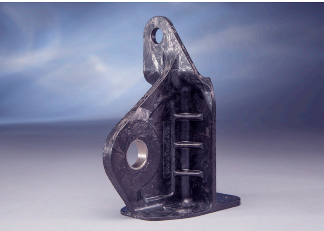
Xycomp® DLF™ complex-shaped component replaces multi-pieced metallic assembly at a fraction of the weight.
