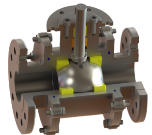
Valve seats
