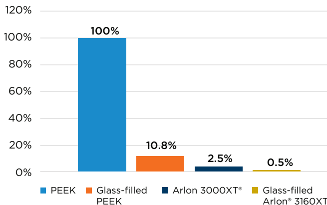
Compressive Creep, 3 Hours @ 500°F, 35,000 psi (260°C, 241 MPa) (Lower Is Better)
