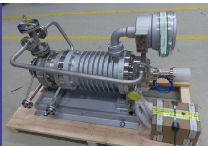
Hermetic Canned Motor Pump
